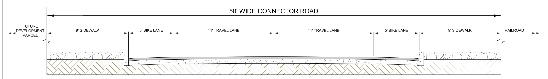
TYPICAL SECTION A-A - PROPOSED CONNECTOR ROAD
